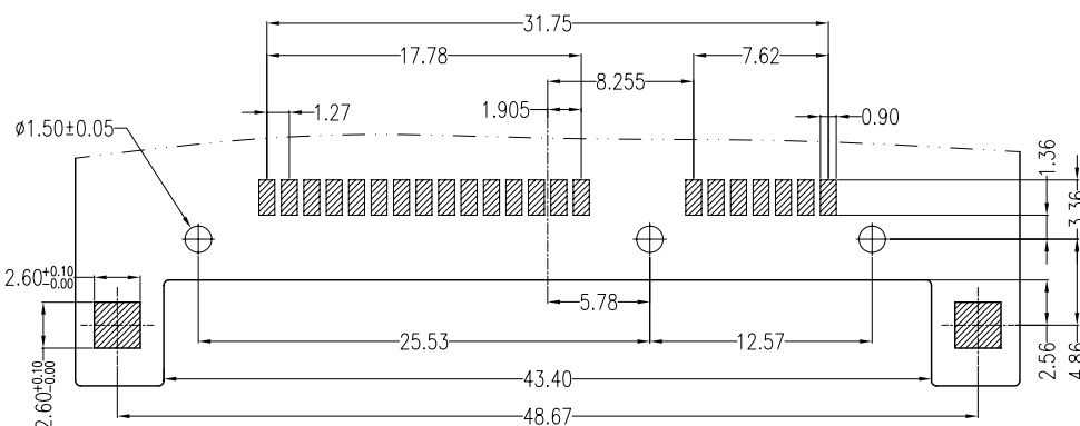
PCB LAYOUT
